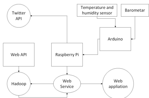
Figure 3: Crowdsensing station for monitoring temperature, humidity and air pressure.
