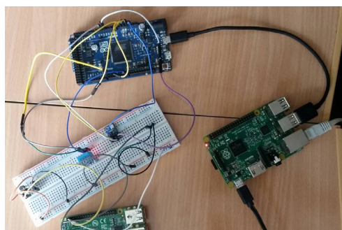
Figure 4: Connected devices in a real environment.
